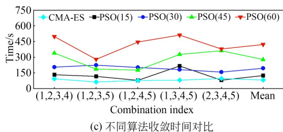
(c) Comparison of convergence time of different algorithms
